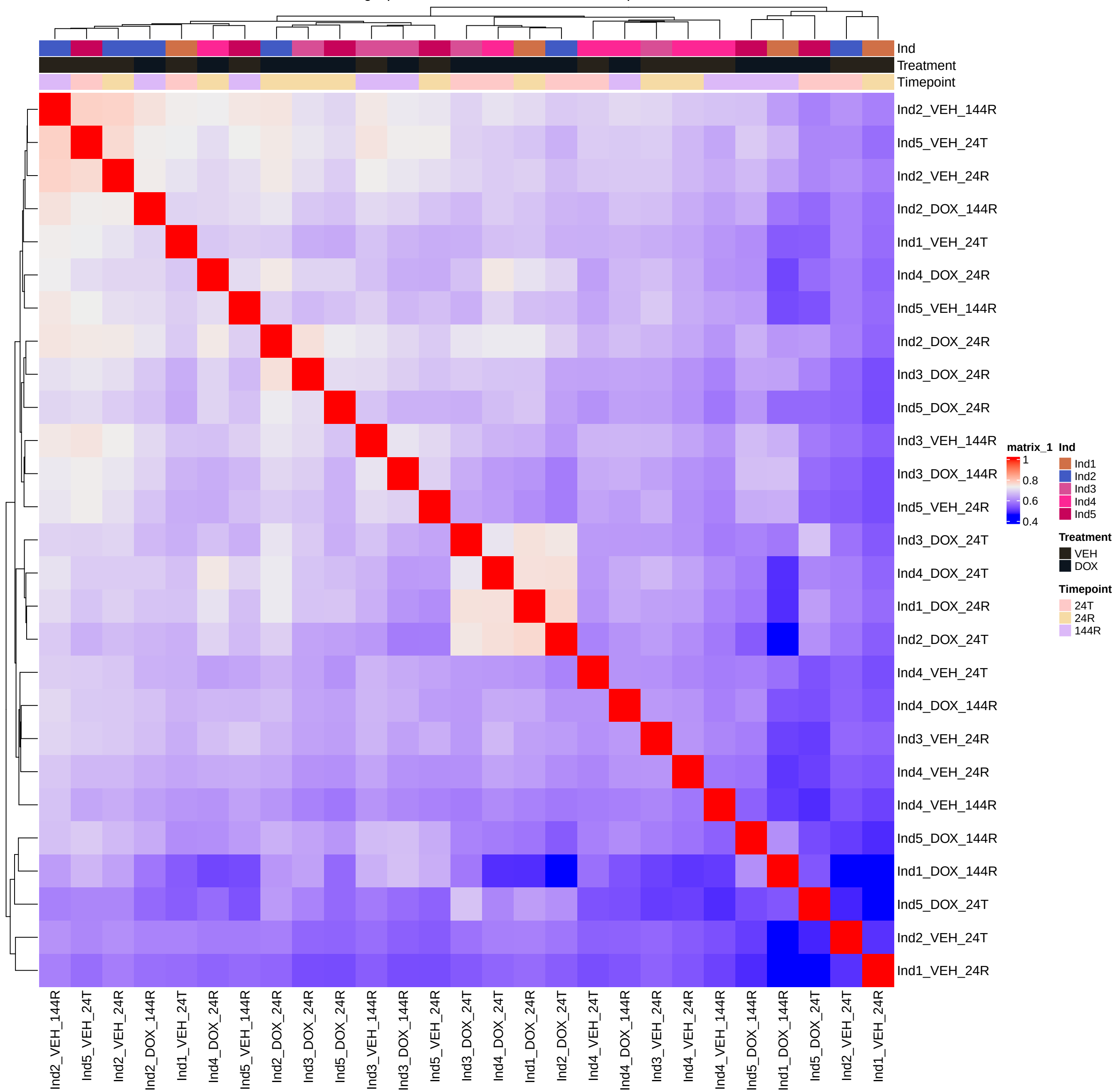
Unfiltered log2cpm H3K36me3 with removal of 1 sample
